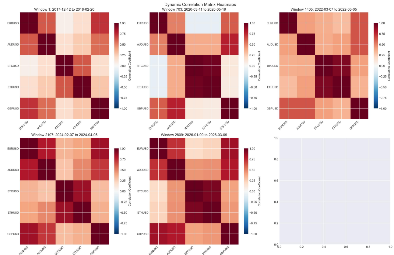
Figure 13: correlation_heatmaps
